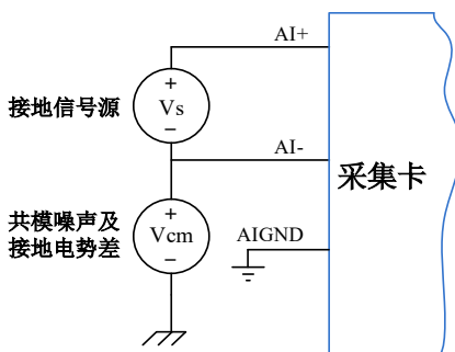
图 4-5-6 接地信号源的差分 (DIFF) 连接
